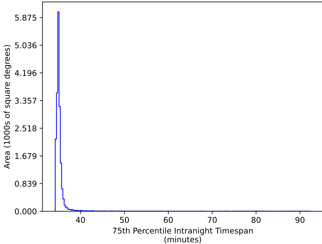
ddf_loaded_fl1_v3.4_10yrs WFD gr bands: 75th Percentile Intranight Timespan
