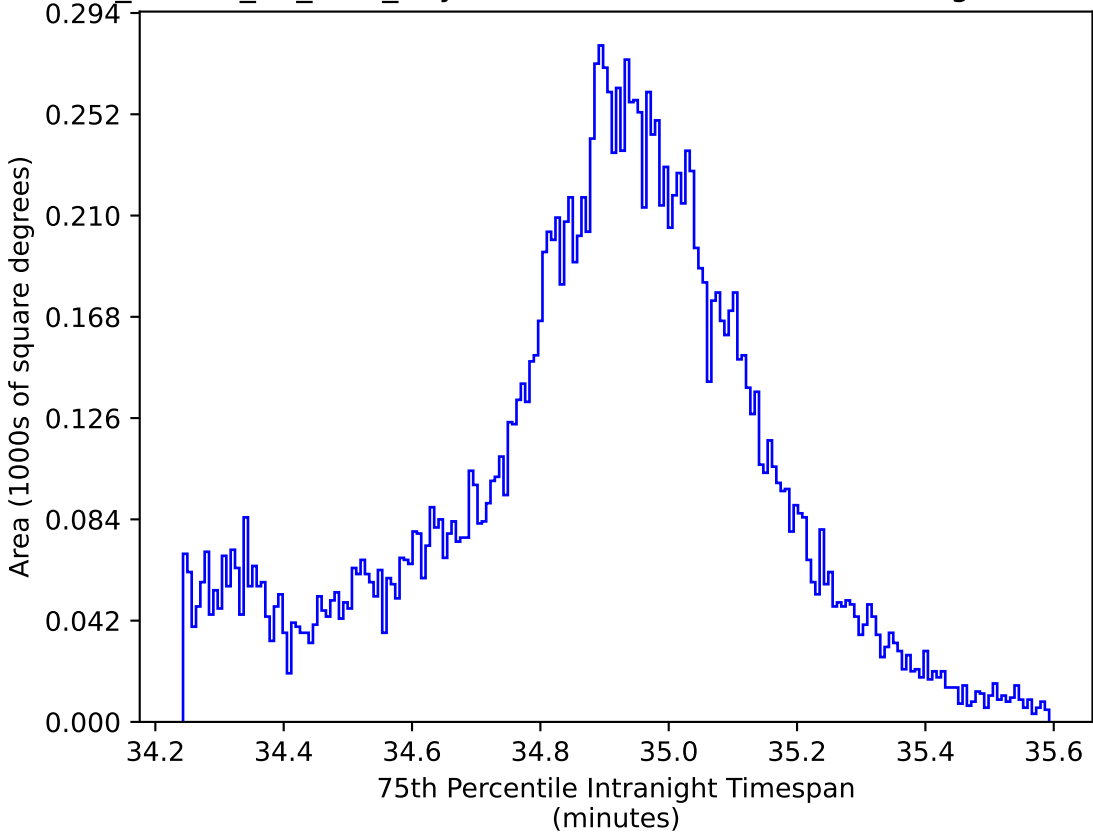
ddf_loaded_fl1_v3.4_10yrs WFD: 75th Percentile Intranight Timespan
