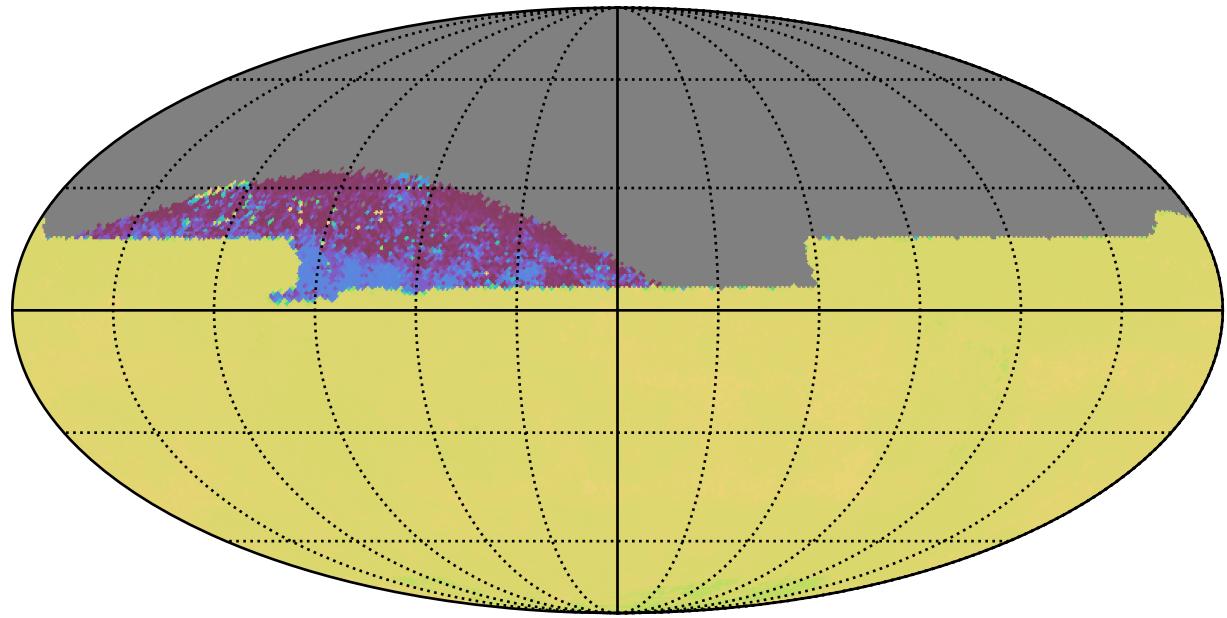
ddf_loaded_fl1_v3.4_10yrs All sky zy bands: 75th Percentile Intranight Timespan
