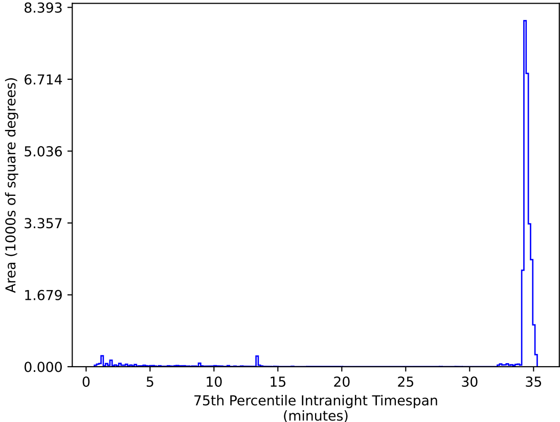
ddf_loaded_fl1_v3.4_10yrs All sky zy bands: 75th Percentile Intranight Timespan
