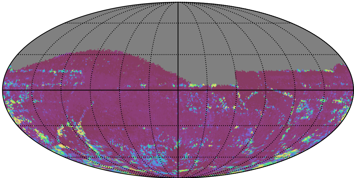
ddf_loaded_fl1_v3.4_10yrs All sky z band: 75th Percentile Intranight Timespan
