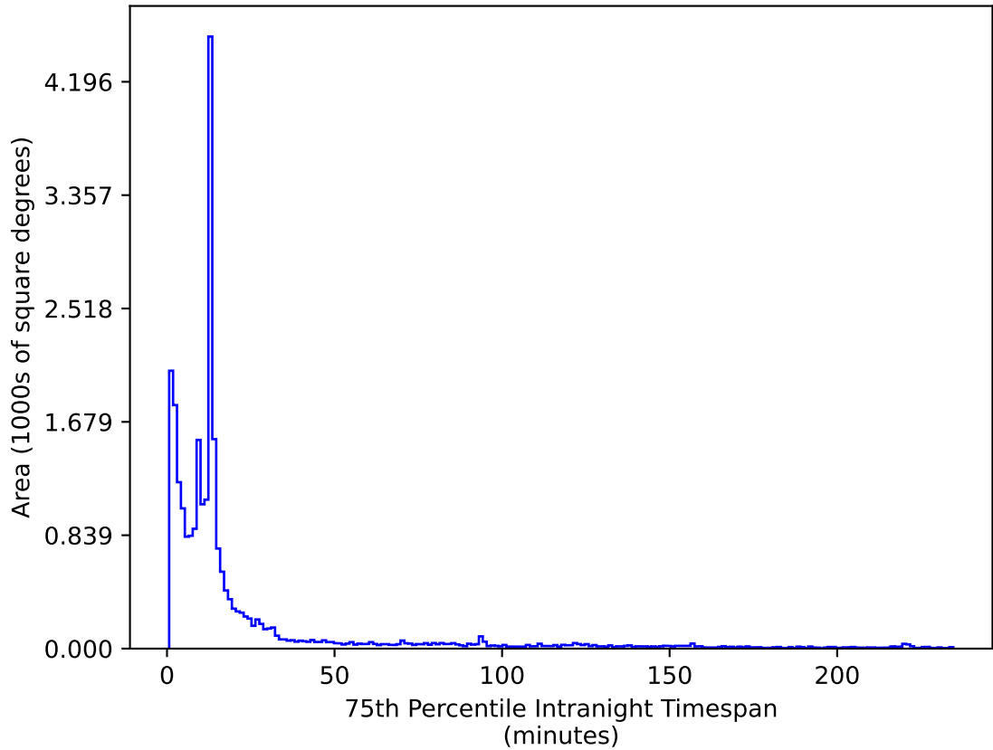
ddf_loaded_fl1_v3.4_10yrs All sky z band: 75th Percentile Intranight Timespan
