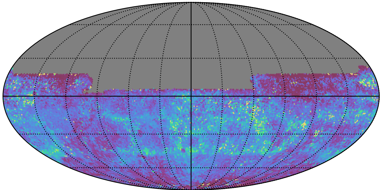
ddf_loaded_fl1_v3.4_10yrs All sky y band: 75th Percentile Intranight Timespan
