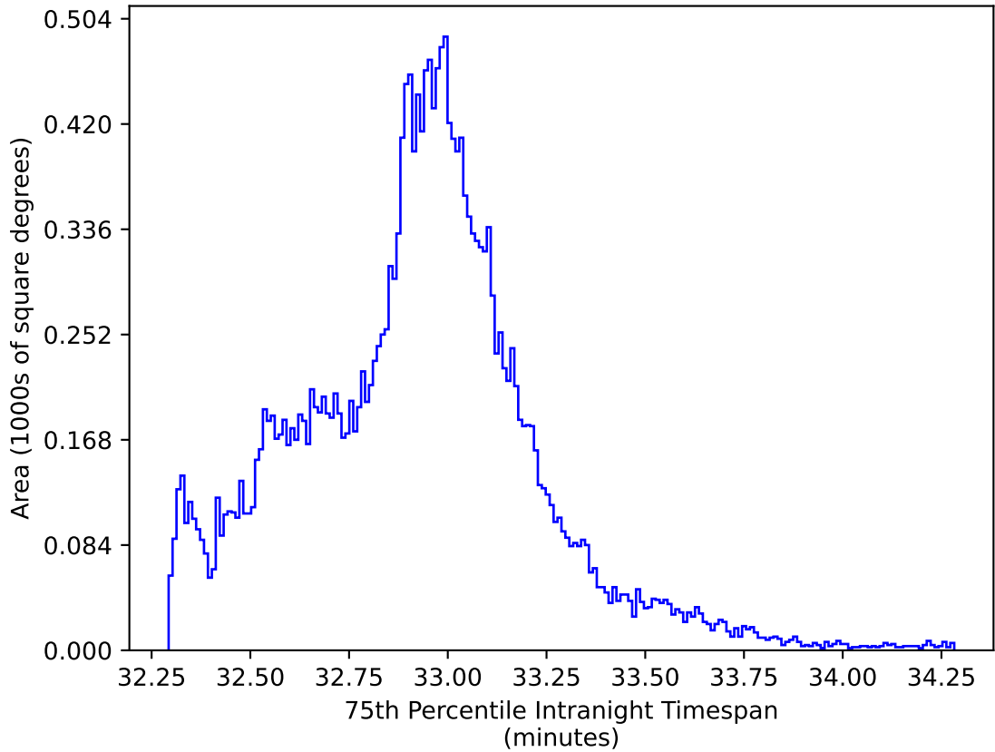
ddf_loaded_fl1_v3.4_10yrs All sky y band: 75th Percentile Intranight Timespan
