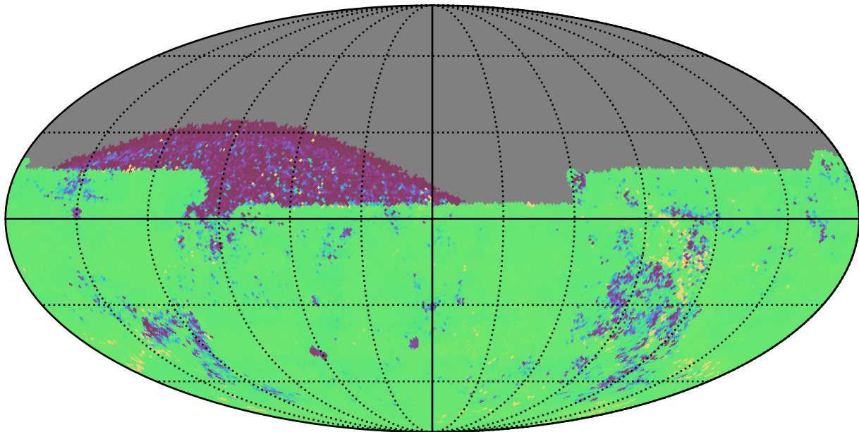
ddf_loaded_fl1_v3.4_10yrs All sky ug bands: 75th Percentile Intranight Timespan
