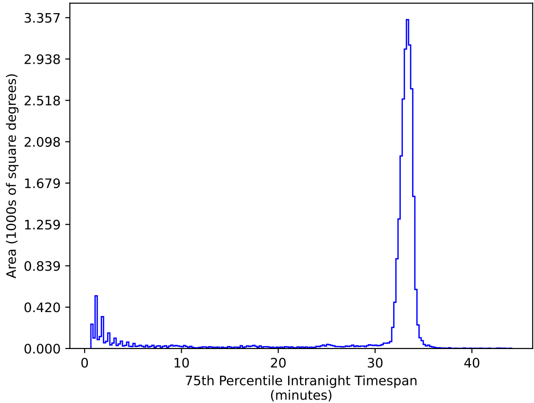
ddf_loaded_fl1_v3.4_10yrs All sky ug bands: 75th Percentile Intranight Timespan
