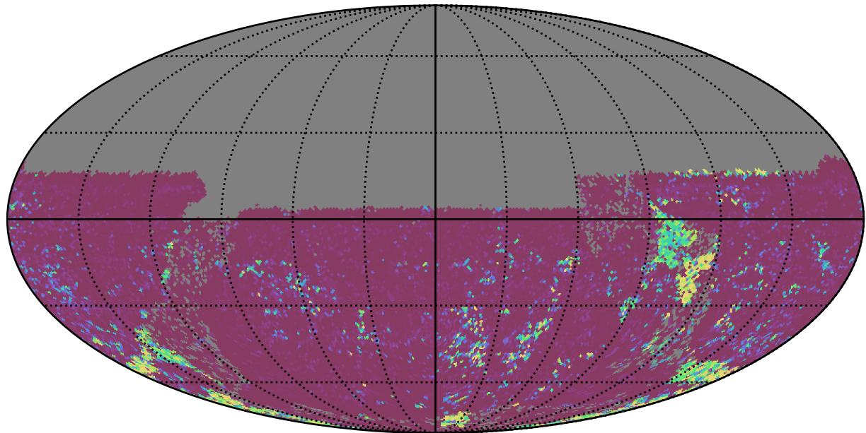
ddf_loaded_fl1_v3.4_10yrs All sky u band: 75th Percentile Intranight Timespan
