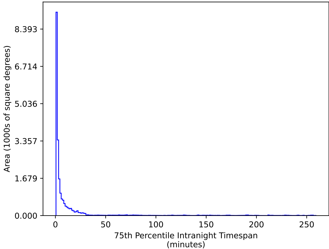
ddf_loaded_fl1_v3.4_10yrs All sky u band: 75th Percentile Intranight Timespan
