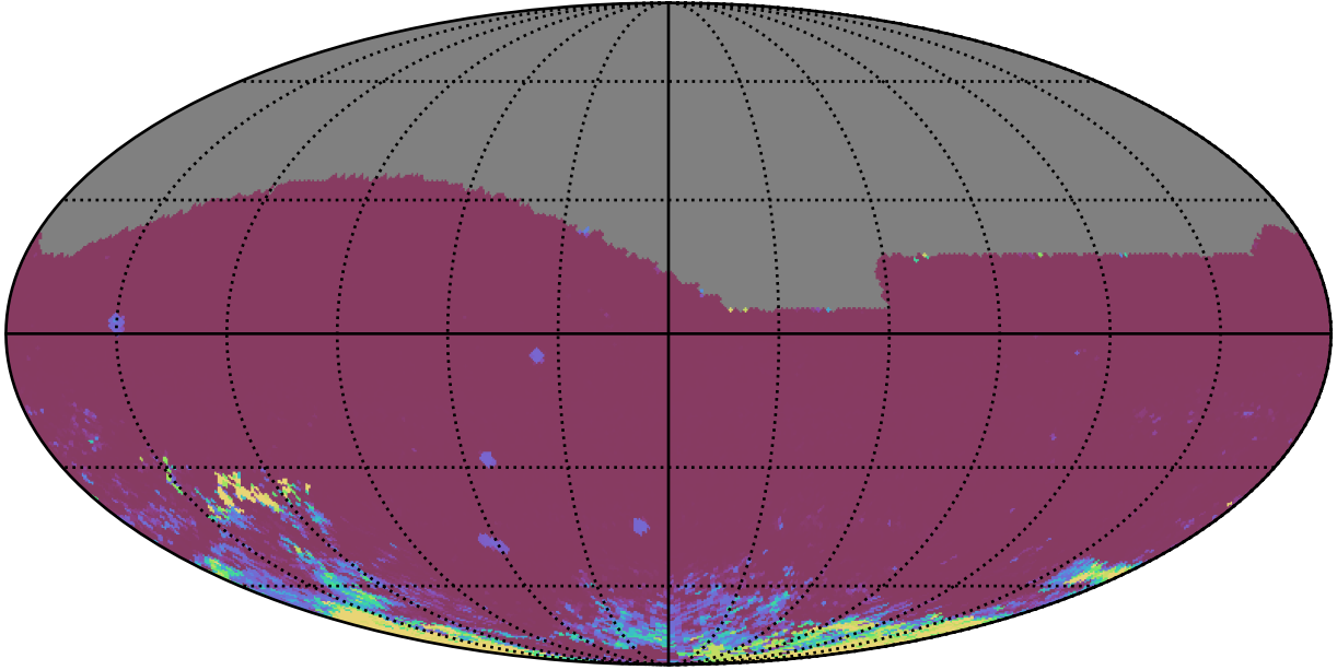
ddf_loaded_fl1_v3.4_10yrs All sky ri bands: 75th Percentile Intranight Timespan
