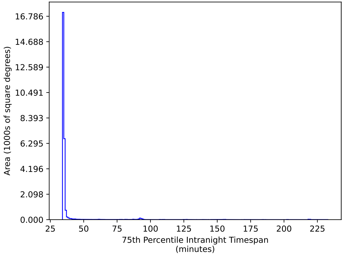
ddf_loaded_fl1_v3.4_10yrs All sky ri bands: 75th Percentile Intranight Timespan
