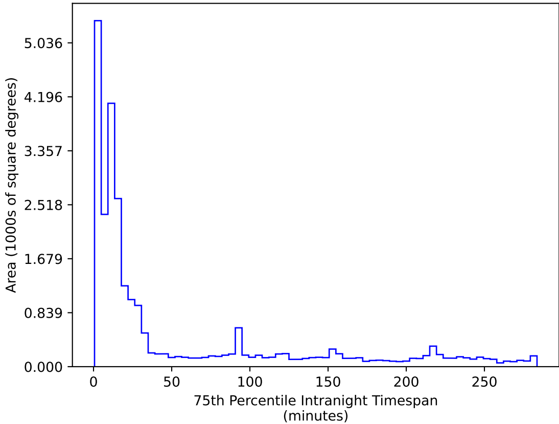
ddf_loaded_fl1_v3.4_10yrs All sky r band: 75th Percentile Intranight Timespan
