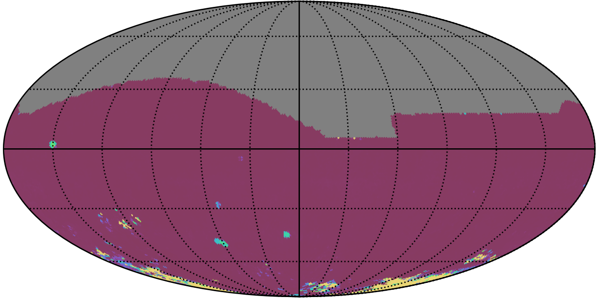
ddf_loaded_fl1_v3.4_10yrs All sky iz bands: 75th Percentile Intranight Timespan
