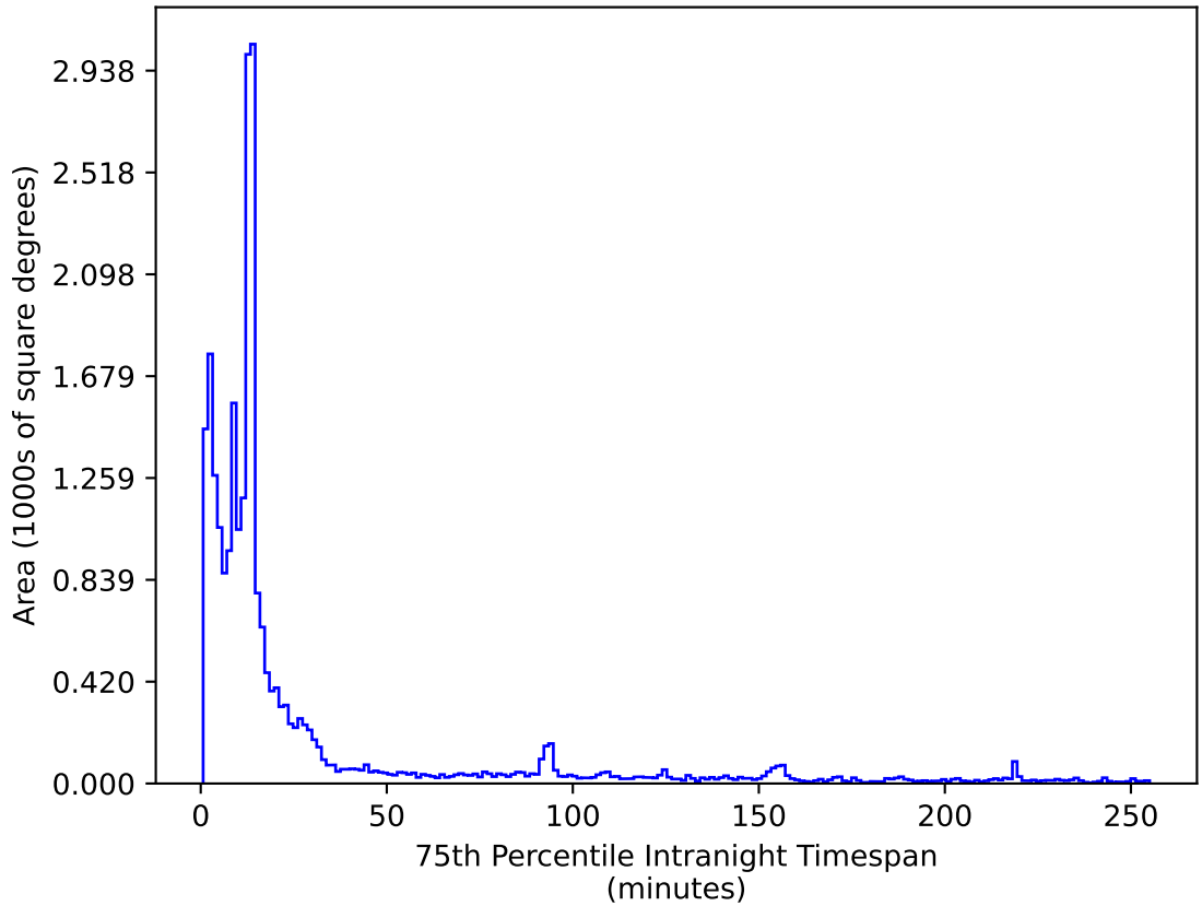
ddf_loaded_fl1_v3.4_10yrs All sky i band: 75th Percentile Intranight Timespan
