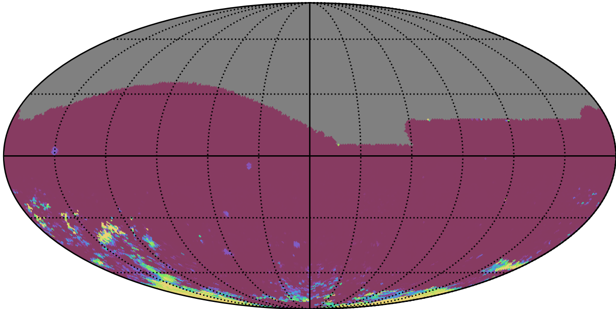
ddf_loaded_fl1_v3.4_10yrs All sky gr bands: 75th Percentile Intranight Timespan
