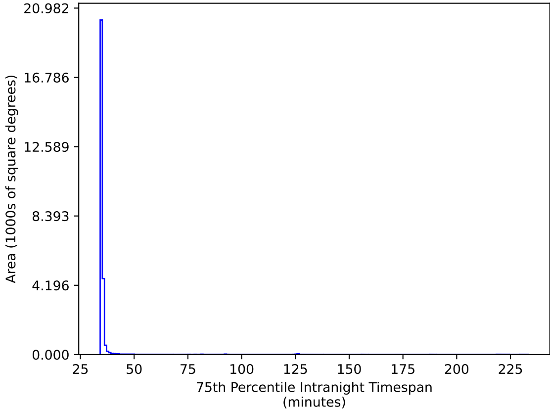
ddf_loaded_fl1_v3.4_10yrs All sky gr bands: 75th Percentile Intranight Timespan
