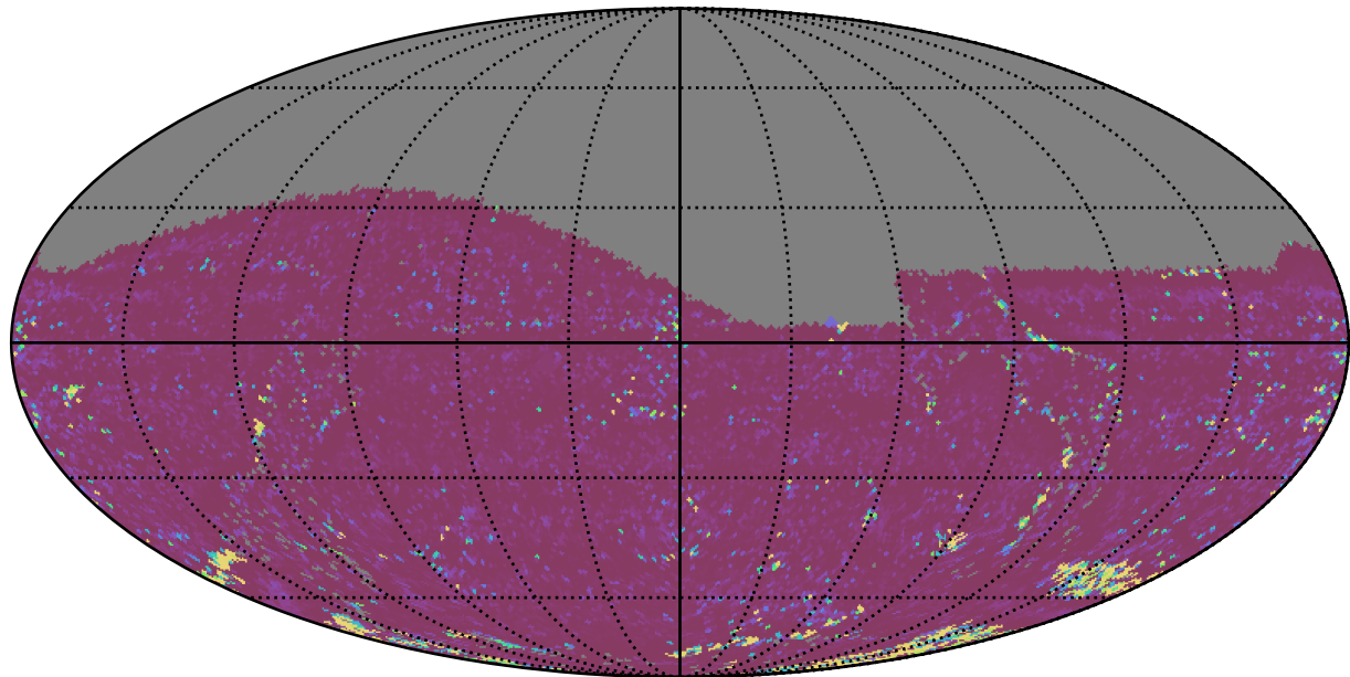
ddf_loaded_fl1_v3.4_10yrs All sky g band: 75th Percentile Intranight Timespan
