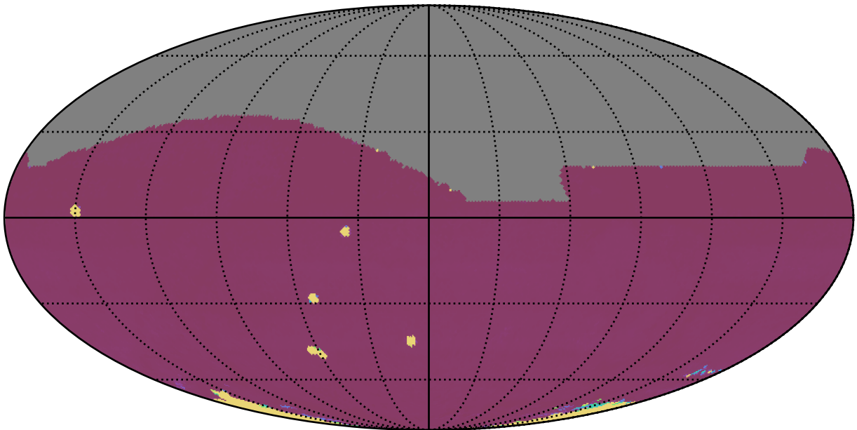
ddf_loaded_fl1_v3.4_10yrs All sky all bands: 75th Percentile Intranight Timespan
