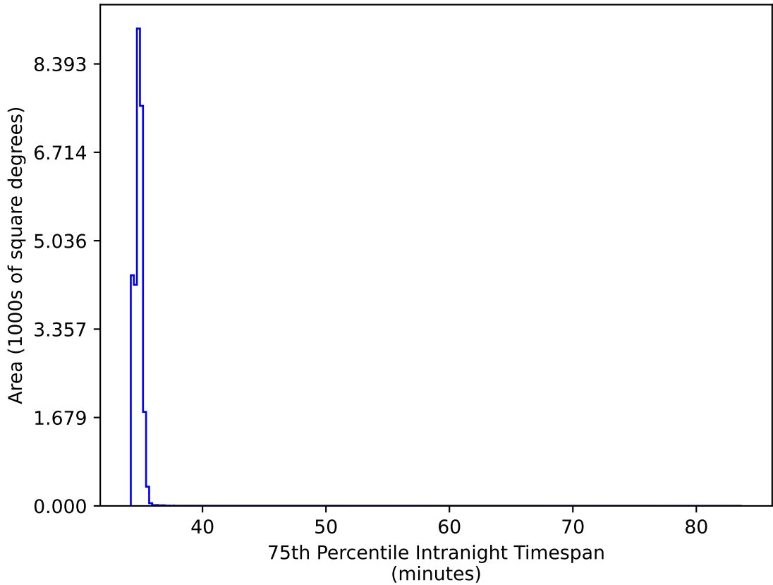
ddf_loaded_fl1_v3.4_10yrs All sky all bands: 75th Percentile Intranight Timespan
