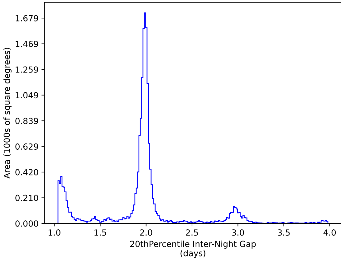
ddf_loaded_fl1_v3.4_10yrs WFD y band: 20thPercentile Inter-Night Gap
