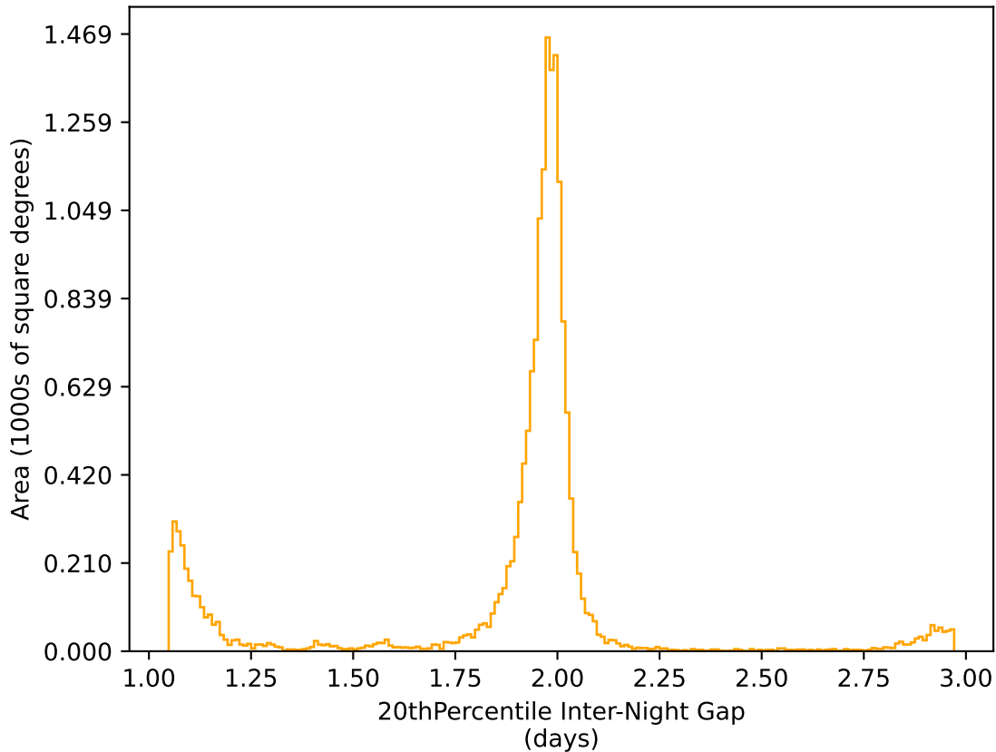
ddf_loaded_fl1_v3.4_10yrs WFD r band: 20thPercentile Inter-Night Gap
