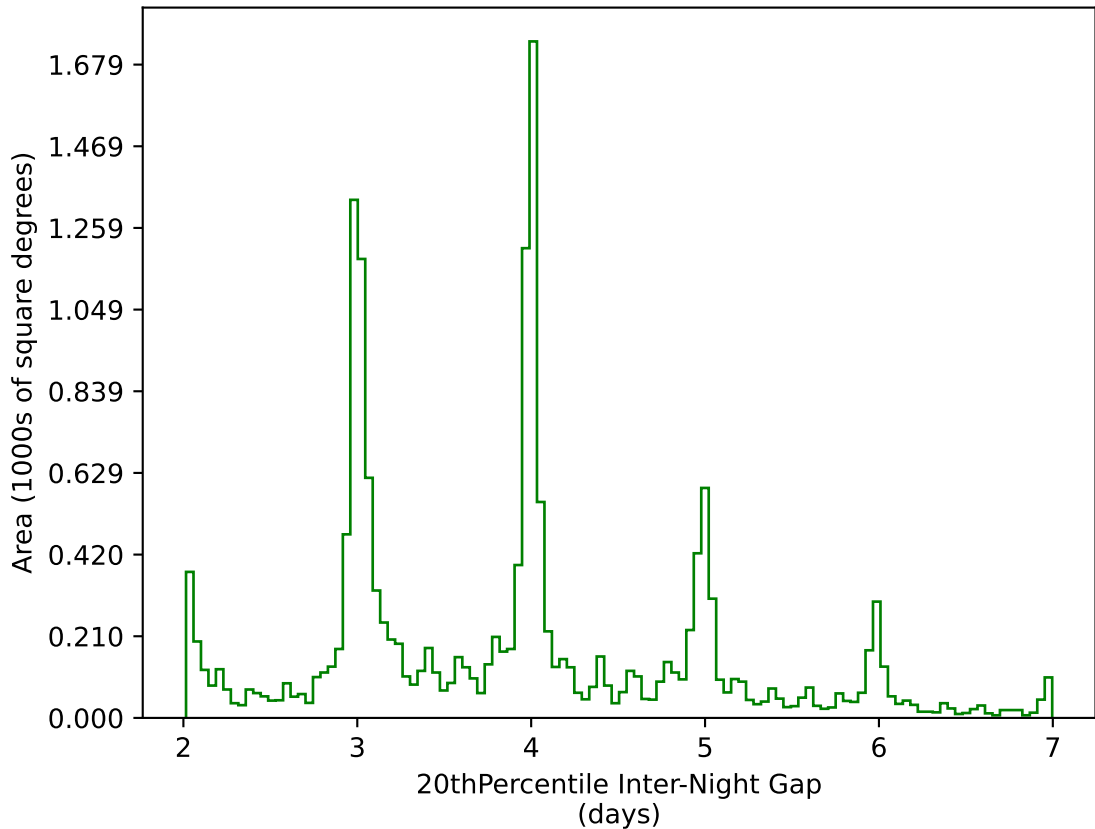
ddf_loaded_fl1_v3.4_10yrs WFD g band: 20thPercentile Inter-Night Gap
