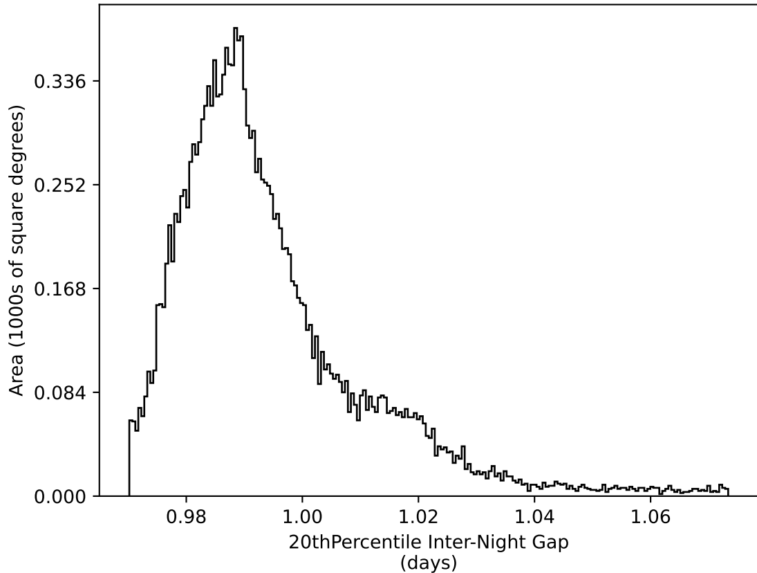
ddf_loaded_fl1_v3.4_10yrs WFD all bands: 20thPercentile Inter-Night Gap
