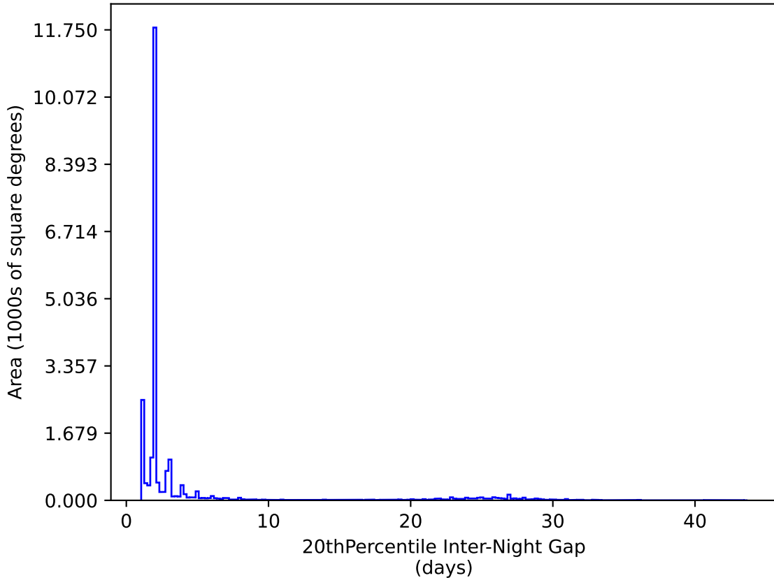
ddf_loaded_fl1_v3.4_10yrs All sky y band: 20thPercentile Inter-Night Gap
