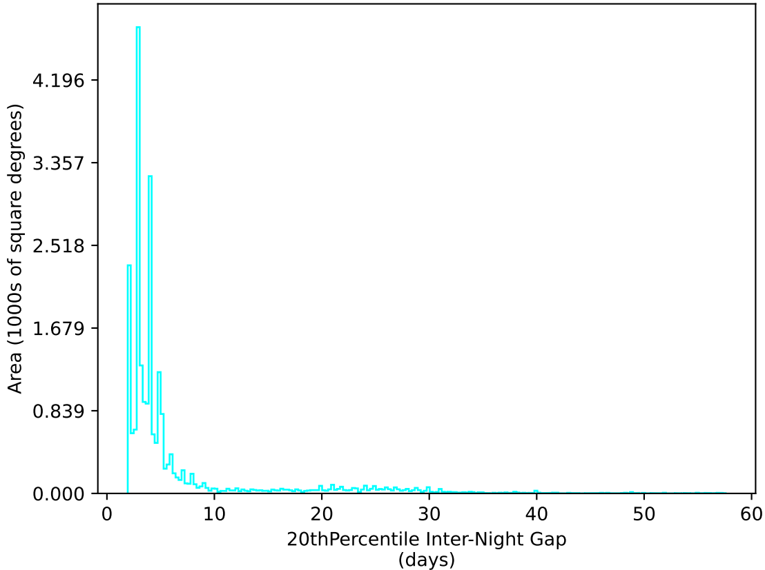
ddf_loaded_fl1_v3.4_10yrs All sky u band: 20thPercentile Inter-Night Gap
