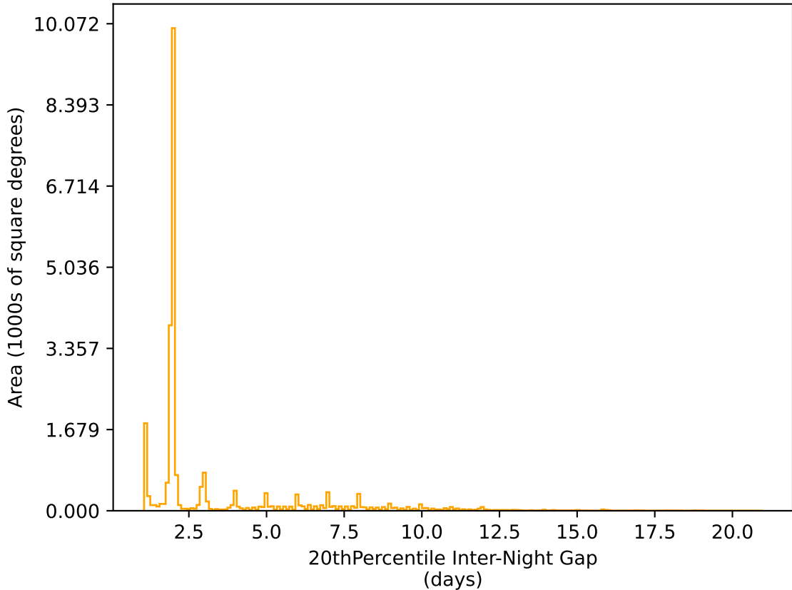
ddf_loaded_fl1_v3.4_10yrs All sky r band: 20thPercentile Inter-Night Gap
