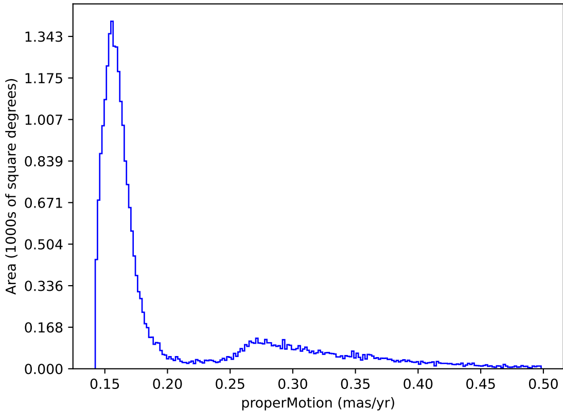
ddf_loaded_fl1_v3.4_10yrs : properMotion
