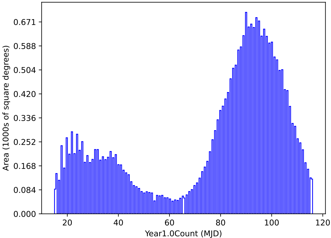
ddf_loaded_fl1_v3.4_10yrs night < 365.25: Year1.0Count
