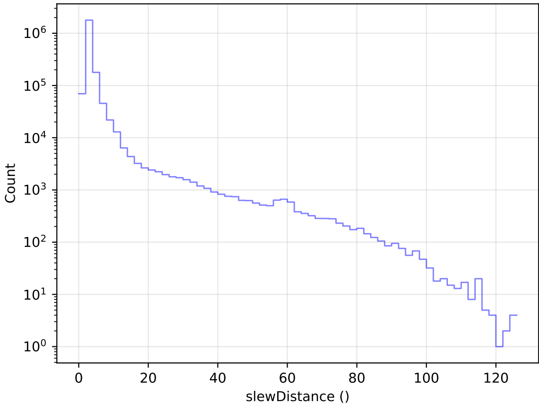
ddf_loaded_fl1_v3.4_10yrs All visits: Slew Distance Histogram
