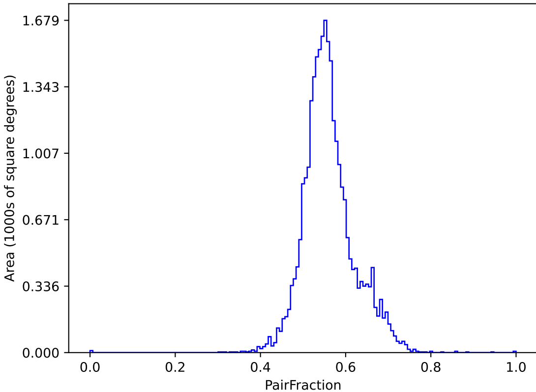
ddf_loaded_fl1_v3.4_10yrs (g or r or i): PairFraction
