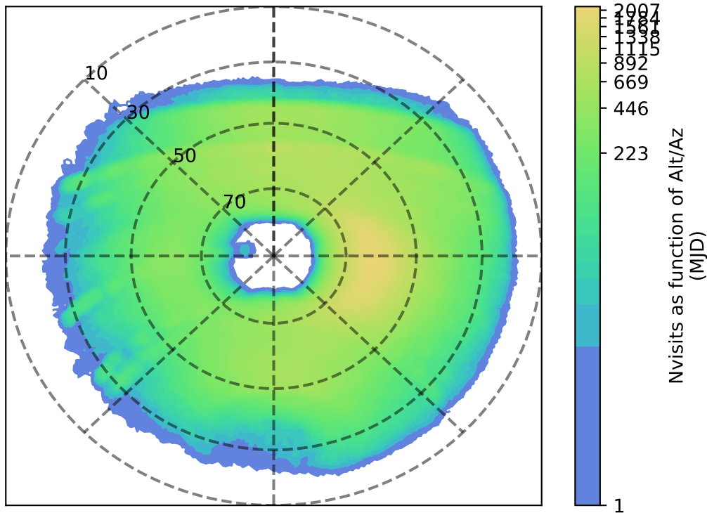
ddf_loaded_fl1_v3.4_10yrs y: Nvisits as function of Alt/Az
