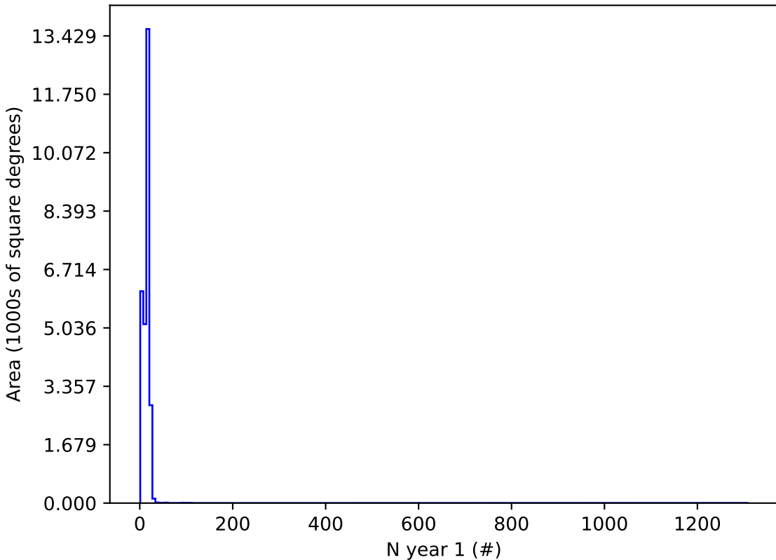
ddf_loaded_fl1_v3.4_10yrs z and night &lt; 365: N year 1
