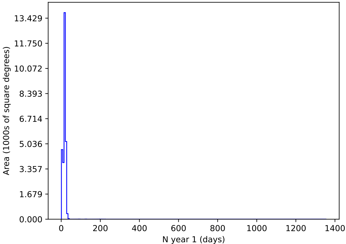
ddf_loaded_fl1_v3.4_10yrs r and night < 365: N year 1
