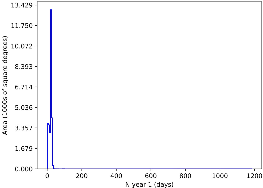
ddf_loaded_fl1_v3.4_10yrs i and night < 365: N year 1
