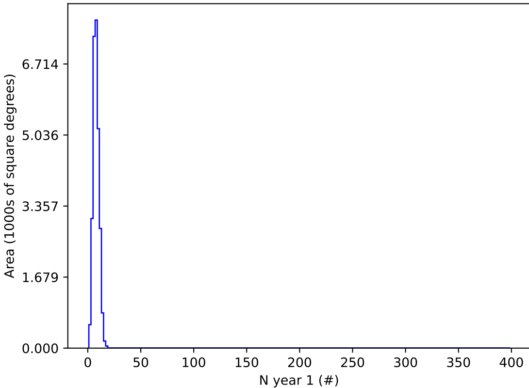
ddf_loaded_fl1_v3.4_10yrs g and night < 365: N year 1
