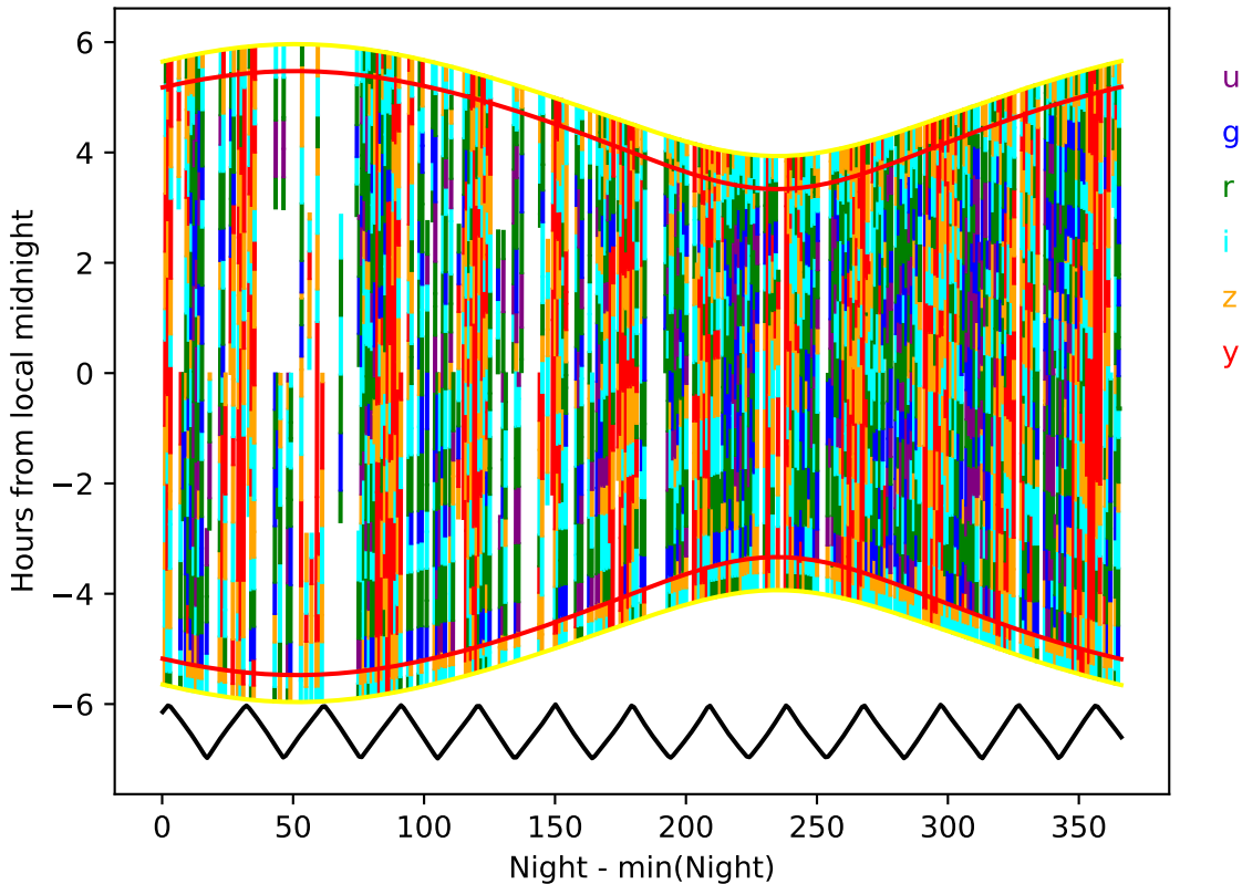
ddf_loaded_fl1_v3.4_10yrs year 9-10: Hourglass
