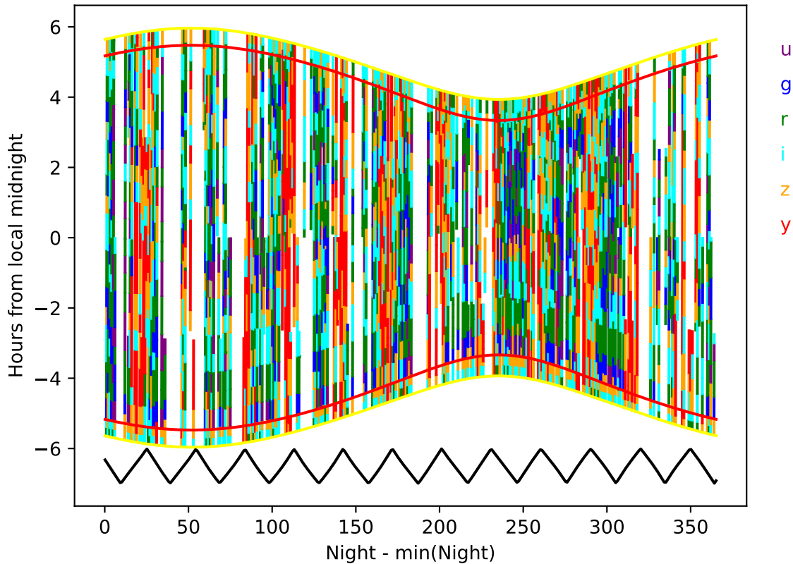
ddf_loaded_fl1_v3.4_10yrs year 7-8: Hourglass
