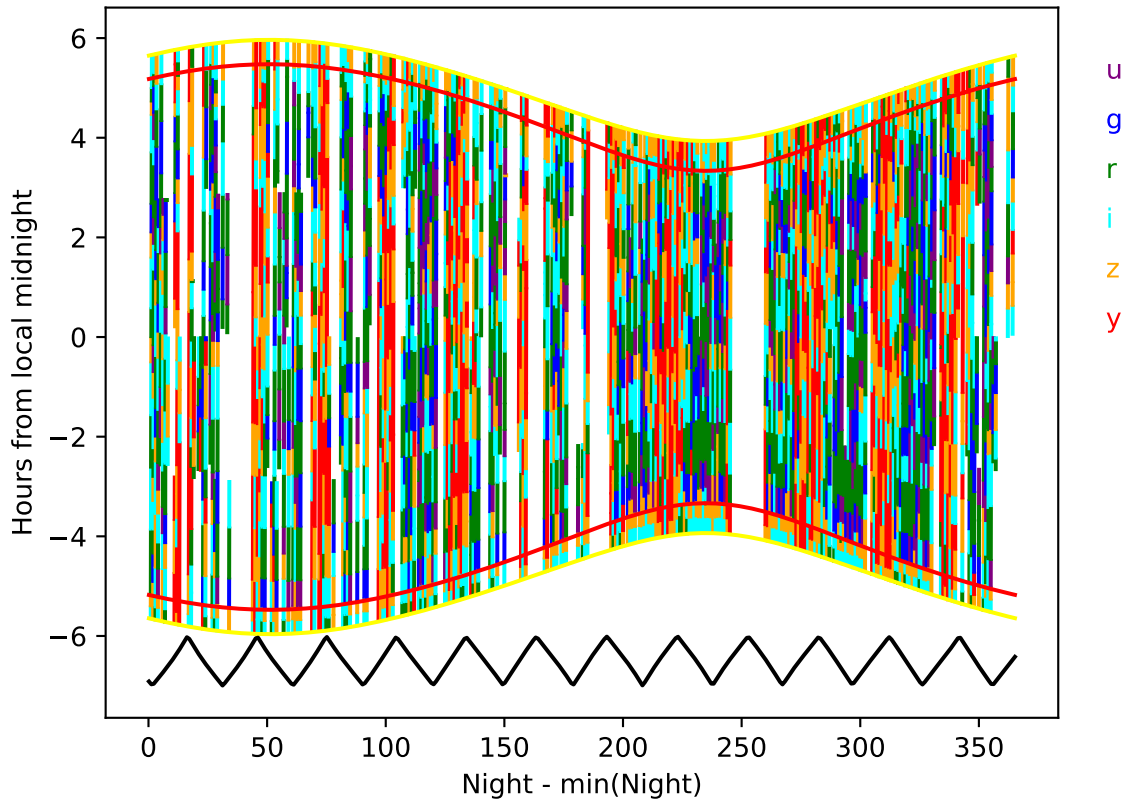
ddf_loaded_fl1_v3.4_10yrs year 5-6: Hourglass
