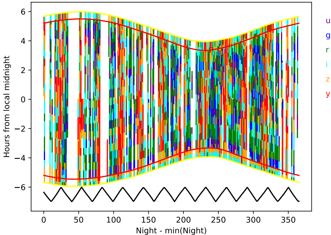
ddf_loaded_fl1_v3.4_10yrs year 4-5: Hourglass
