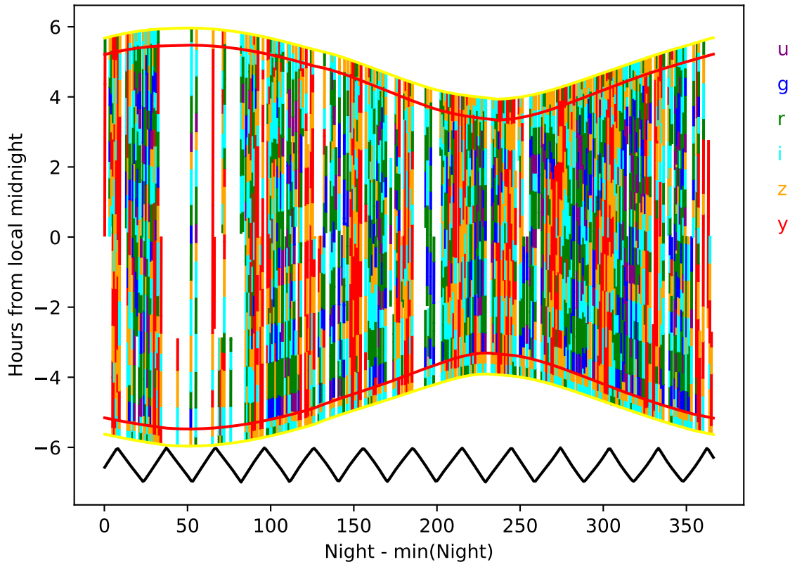
ddf_loaded_fl1_v3.4_10yrs year 3-4: Hourglass
