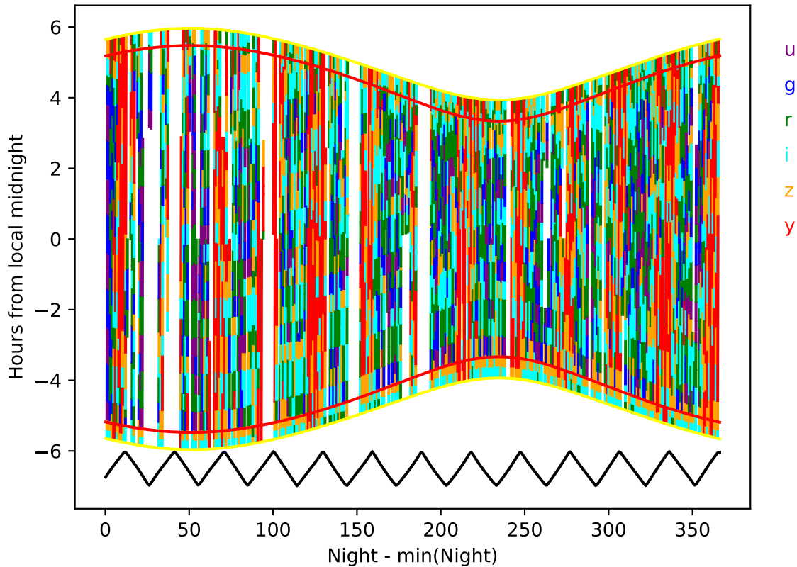
ddf_loaded_fl1_v3.4_10yrs year 0-1: Hourglass
