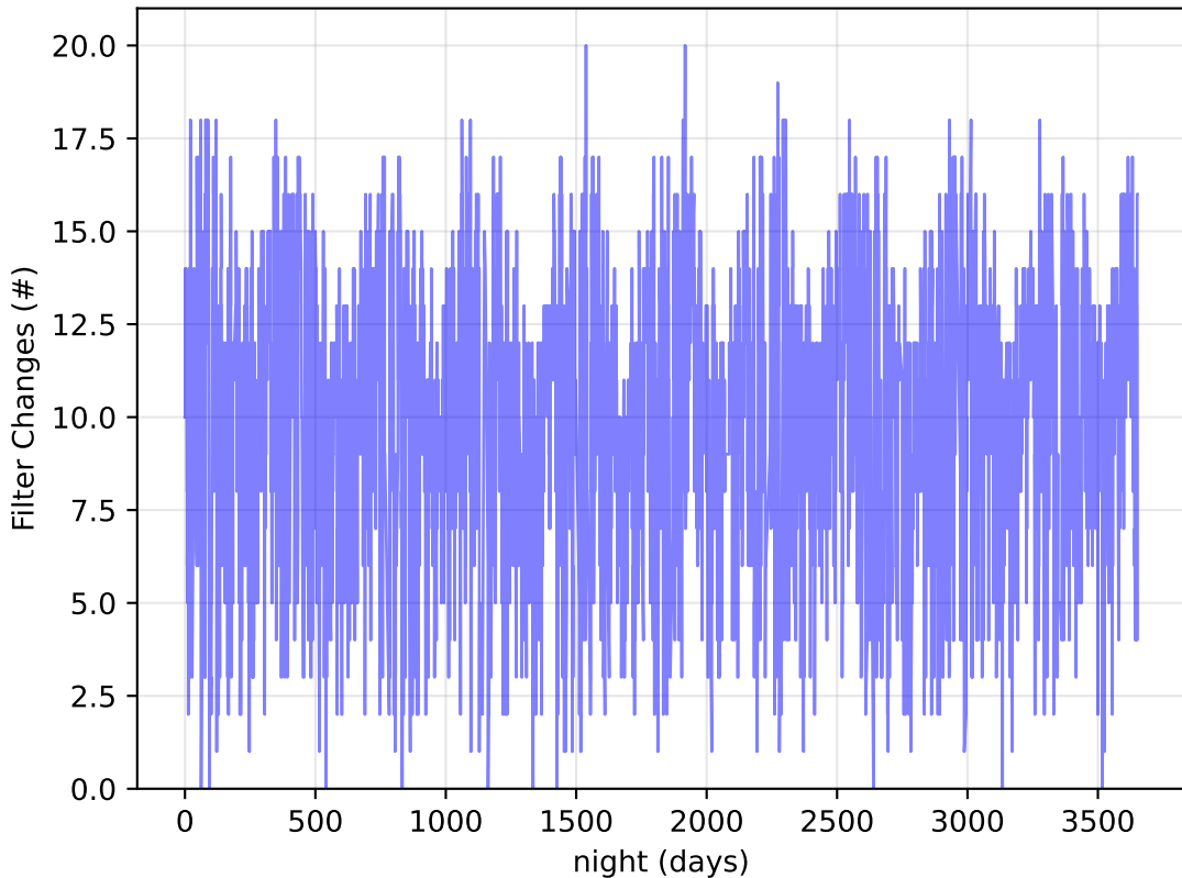
ddf_loaded_fl1_v3.4_10yrs : Filter Changes
