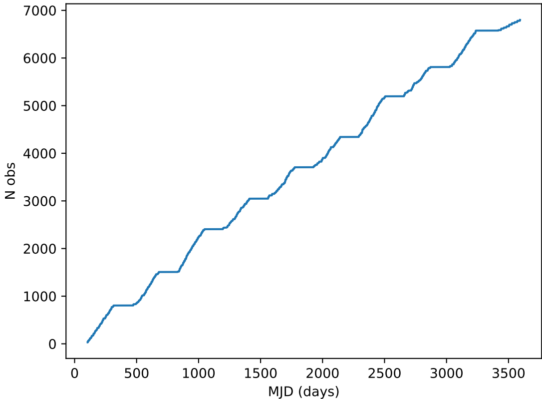
ddf_loaded_fl1_v3.4_10yrs note like DD:EDFS_b%: Cumulative
