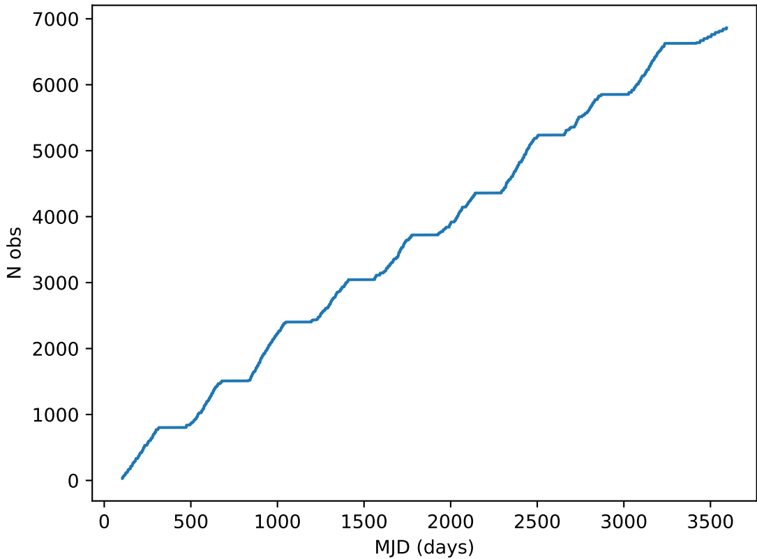
ddf_loaded_fl1_v3.4_10yrs note like DD:EDFS_a%: Cumulative
