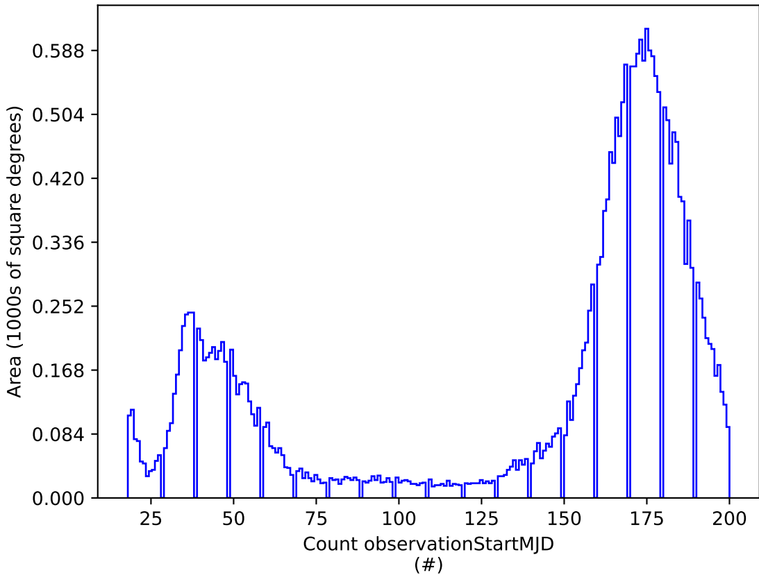
ddf_loaded_fl1_v3.4_10yrs z: Count observationStartMJD
