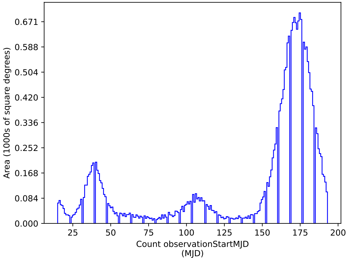
ddf_loaded_fl1_v3.4_10yrs y: Count observationStartMJD
