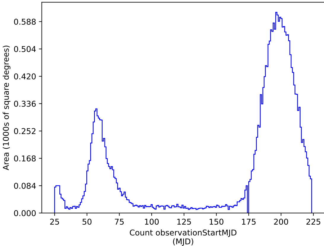
ddf_loaded_fl1_v3.4_10yrs i: Count observationStartMJD
